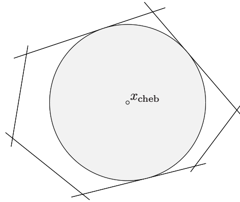
Figure 8.5 Chebyshev center of a polyhedron C , in the Euclidean norm. The center x_{\text{cheb}} is the deepest point inside C , in the sense that it is farthest from the exterior, or complement, of C . The center x_{\text{cheb}} is also the center of the largest Euclidean ball (shown lightly shaded) that lies inside C .
