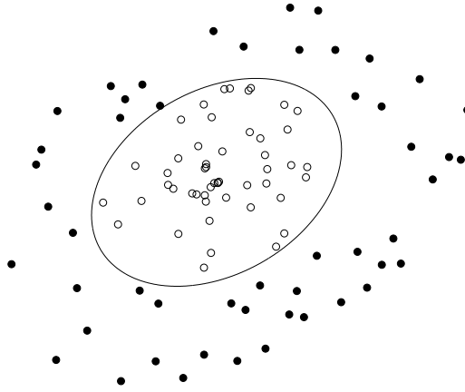
Figure 8.13 Quadratic discrimination, with the condition that P \prec 0 . This means that we seek an ellipsoid containing all of x_i (shown as open circles) and none of the y_i (shown as filled circles). This can be solved as an SDP feasibility problem.
