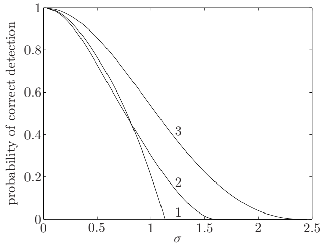
Figure 7.6 Chebyshev lower bounds on the probability of correct detection for symbols s_1 , s_2 , and s_3 . These bounds are valid for any noise distribution that has zero mean and covariance \sigma^2 I .
