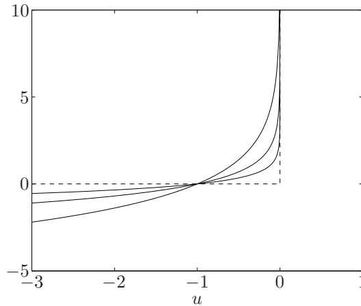
Figure 11.1 The dashed lines show the function I_-(u) , and the solid curves show \widehat{I}_-(u) = -(1/t)\log(-u) , for t = 0.5, 1, 2 . The curve for t = 2 gives the best approximation.
